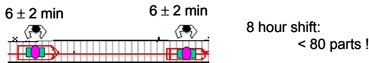
Figure 3. Two-worker assembly line, variable process times
